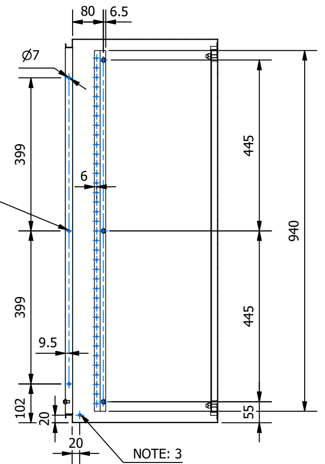
SECTION E-E
