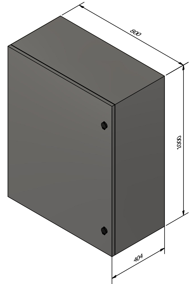
ISOMETRIC VIEW
