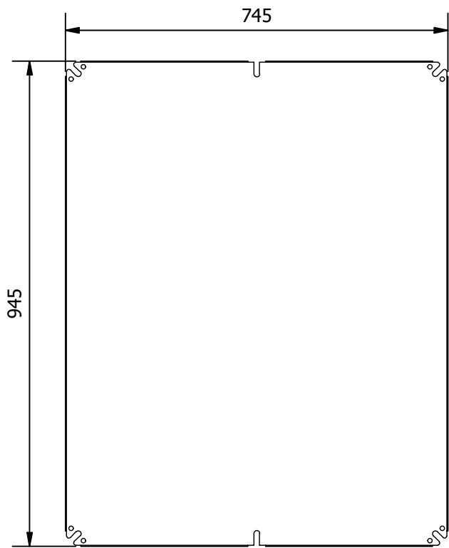
GEAR TRAY
