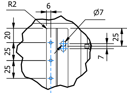
DETAIL F
