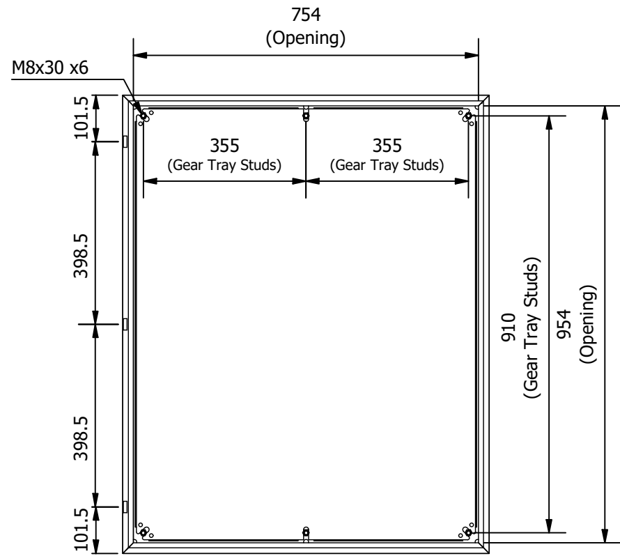
FRONT VIEW WITHOUT DOOR
