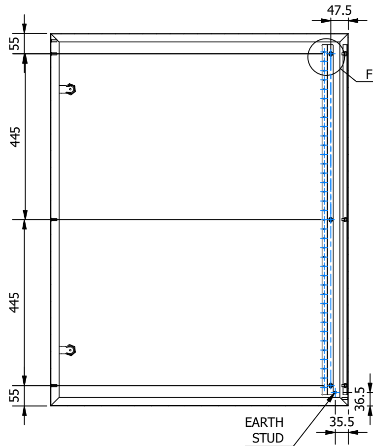
SECTION C-C
