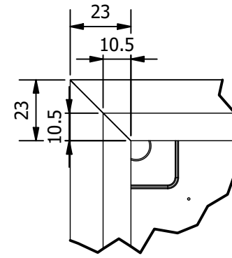
DETAIL G
